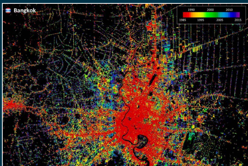
Figure 14: WSF Evolution of Bangkok region, Thailand. Red corresponds to the urban extent in 1985 and yellow-green-blue indicates the growth to 2015. Credit: DLR
