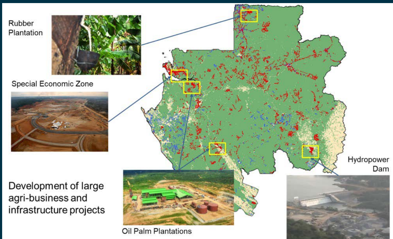
Figure 18: Extent of forest in Gabon in 2015 and main causes of deforestation. Credit: Christophe Sannier
