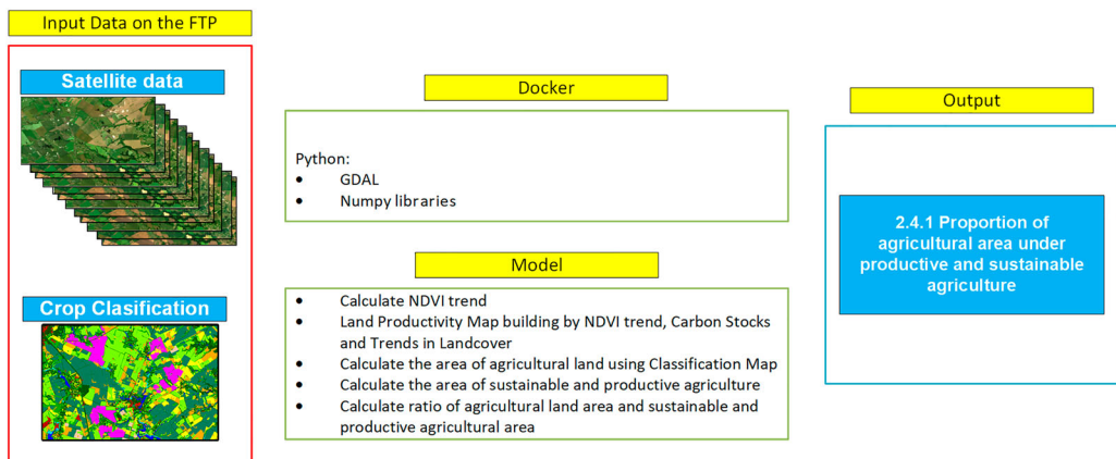
Figure 5. Workflow for indicator 2.4.1 implementation in VLab.
