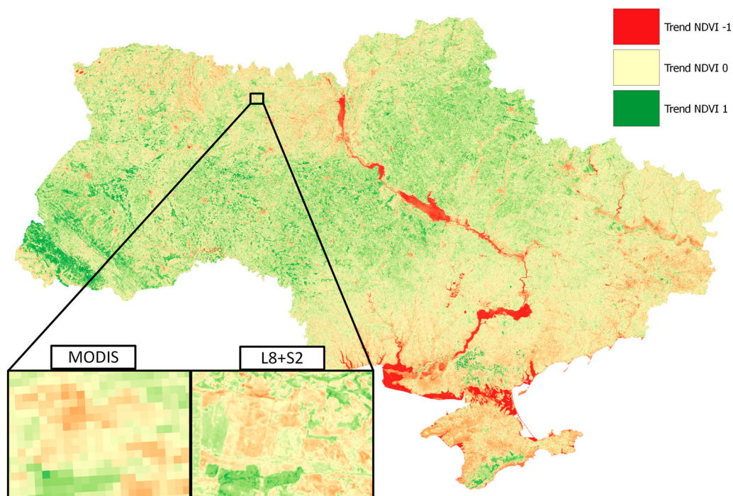
Figure 9. Comparison coarse resolution productivity map based on MODIS data and our high-resolution productivity map for Ukraine territory for the year 2017.
