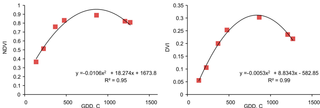
Figure 7. Examples of VIs (NDVI and DVI) fitting versus accumulated GDD for a winter wheat field in 2017.
