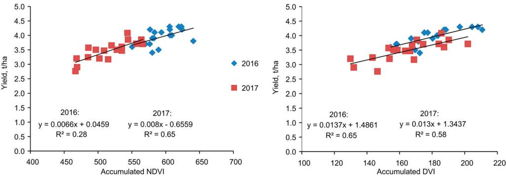
Figure 8. Relationship between accumulated NDVI and DVI against winter wheat yields for 2016 and 2017.
