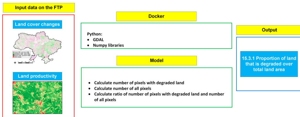
Figure 6. Workflow for indicator 15.3.1 realisation in VLab.
