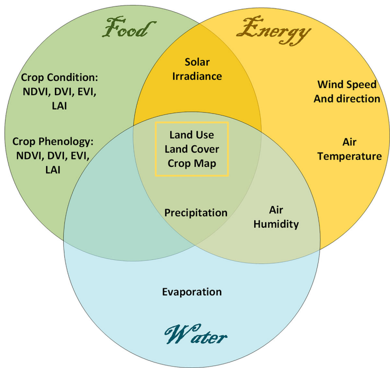
Figure 2. Food, water, energy Essential Variables that are used in SDG indicator 15.1.1, 15.3.1, 2.4.1 workflows.
